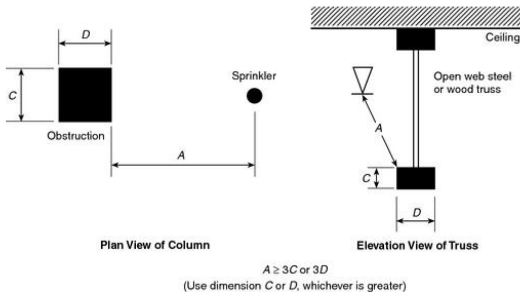
FIGURE 8.11.5.2.1.3 Minimum Distance from Obstruction (Large Drop Sprinkler).
