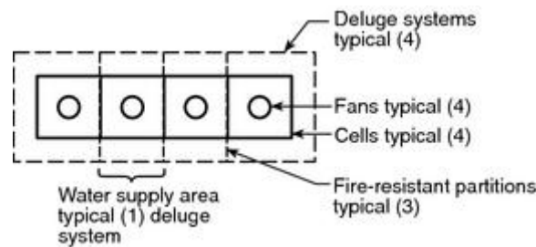
FIGURE A.21.24.1.7.1.3 Multiple Deluge Systems. [214:Figure A.5.6.1.3]
