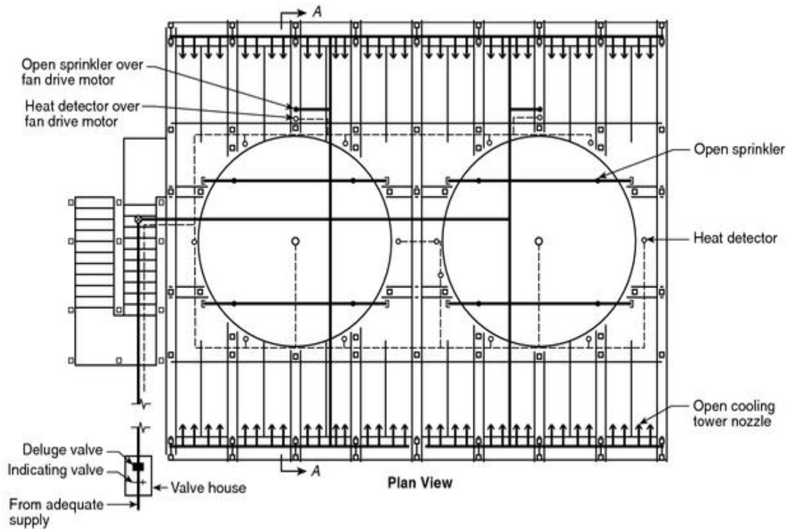
FIGURE A.21.24.2(c) Plan View, Typical Deluge Fire Protection Arrangement for Multicell Crossflow Towers. [214:Figure A.5.2.4.2(c)]
