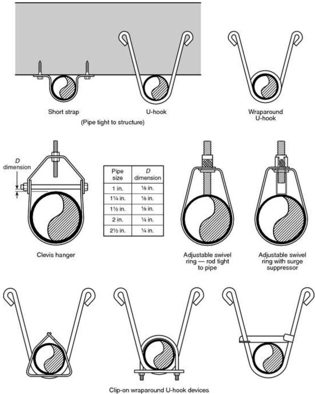
FIGURE A.9.2.3.4(b) Examples of Acceptable Hangers for End-of-Line (or Armover) Pendent Sprinklers.
