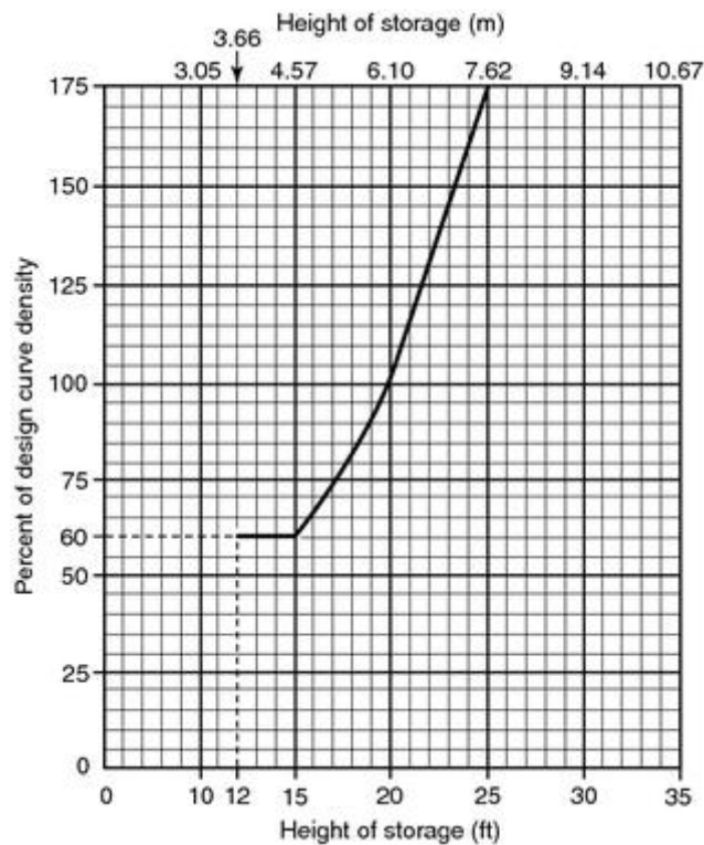
FIGURE 16.2.1.3.4.1 Ceiling Sprinkler Density vs. Storage Height.
