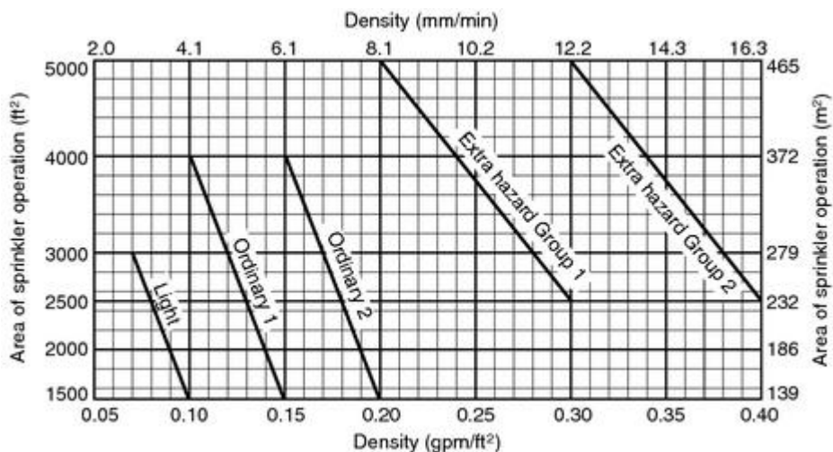
FIGURE 11.2.3.1.1 Density/Area Curves.
