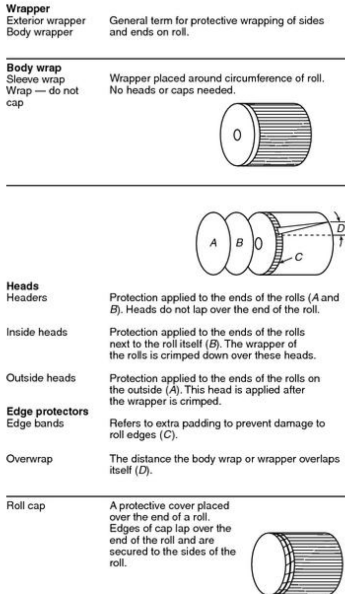
FIGURE A.3.9.5.6.3 Wrapping and Capping Terms and Methods.
