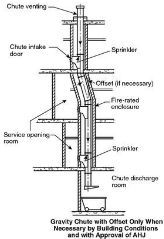
FIGURE A.21.16.2.1(b) Gravity Waste Chute. [82:Figure A.5.2(b)]
