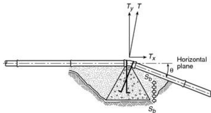
FIGURE A.10.8.2(b) Bearing Thrust Block. [24:Figure A.10.8.2(b)]
