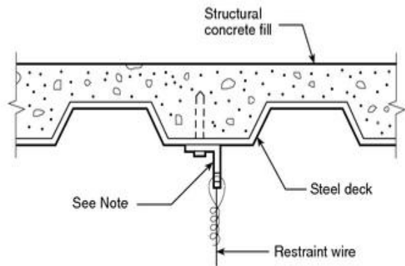
Note: See Figure A.9.3.6.1(a), Detail A. Detail D — At steel deck with concrete fill
