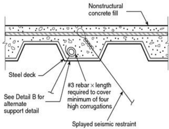
Detail A — At steel deck with insulating fill
