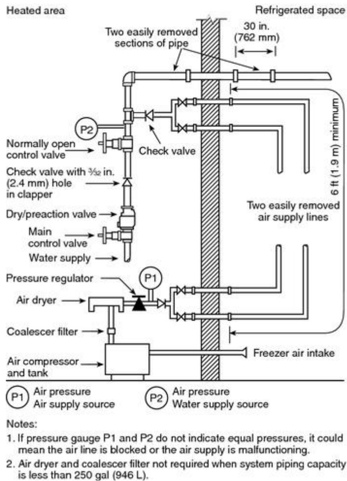
FIGURE A.7.9.2.4 Refrigerator Area Sprinkler Systems Used to Minimize the Chances of Developing Ice Plugs.
